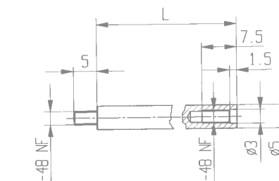
Contact Point Extensions
